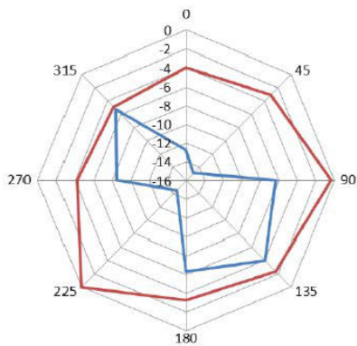
Blue - Whip 153MHz Red - Patch
