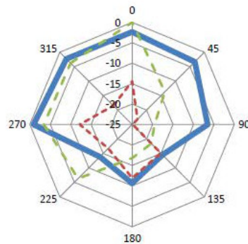
Blue - Patch 2.4GHz Red - COTS Dipole Green - COTS 8.5 dBi
