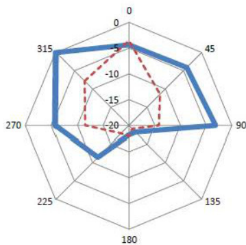
Blue - Patch 5.5GHz Red - COTS 6 dBi
