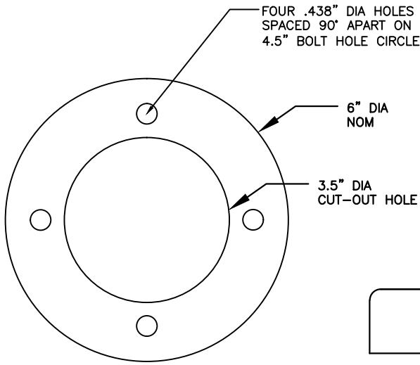
BOLT HOLE MOUNTING PATTERN
